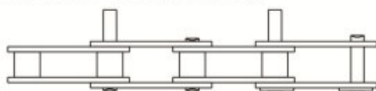
每两节一根长销 D2 each two links one extended pin
