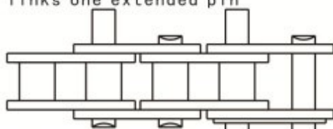
每两节一根长销 D2 each two links one extended pin
