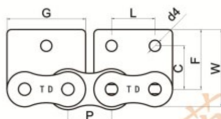
单侧 SWA-1SWA-2 Unilateral
