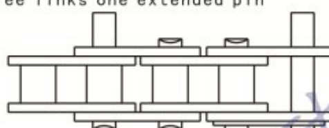
每三节一根长销 D3 each three links one extended pin
